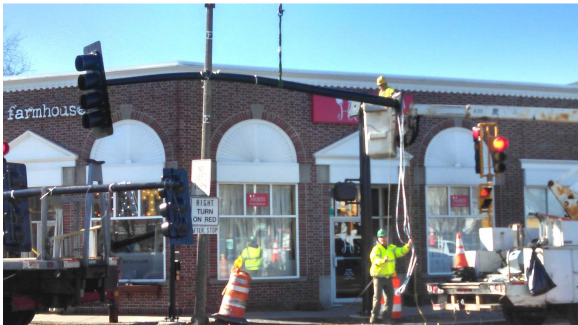
Installing the mast arm on the southwest corner of Great Plain Ave. and Dedham Ave.
