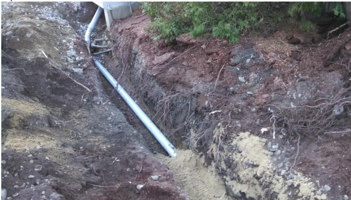
3 inch schedule 80 PVC conduit being installed to existing controller in MBTA property also showing existing cables near controller
